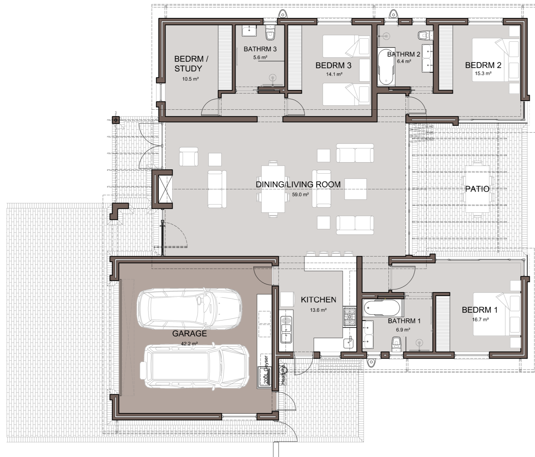
1: 100 FLOOR PLAN
