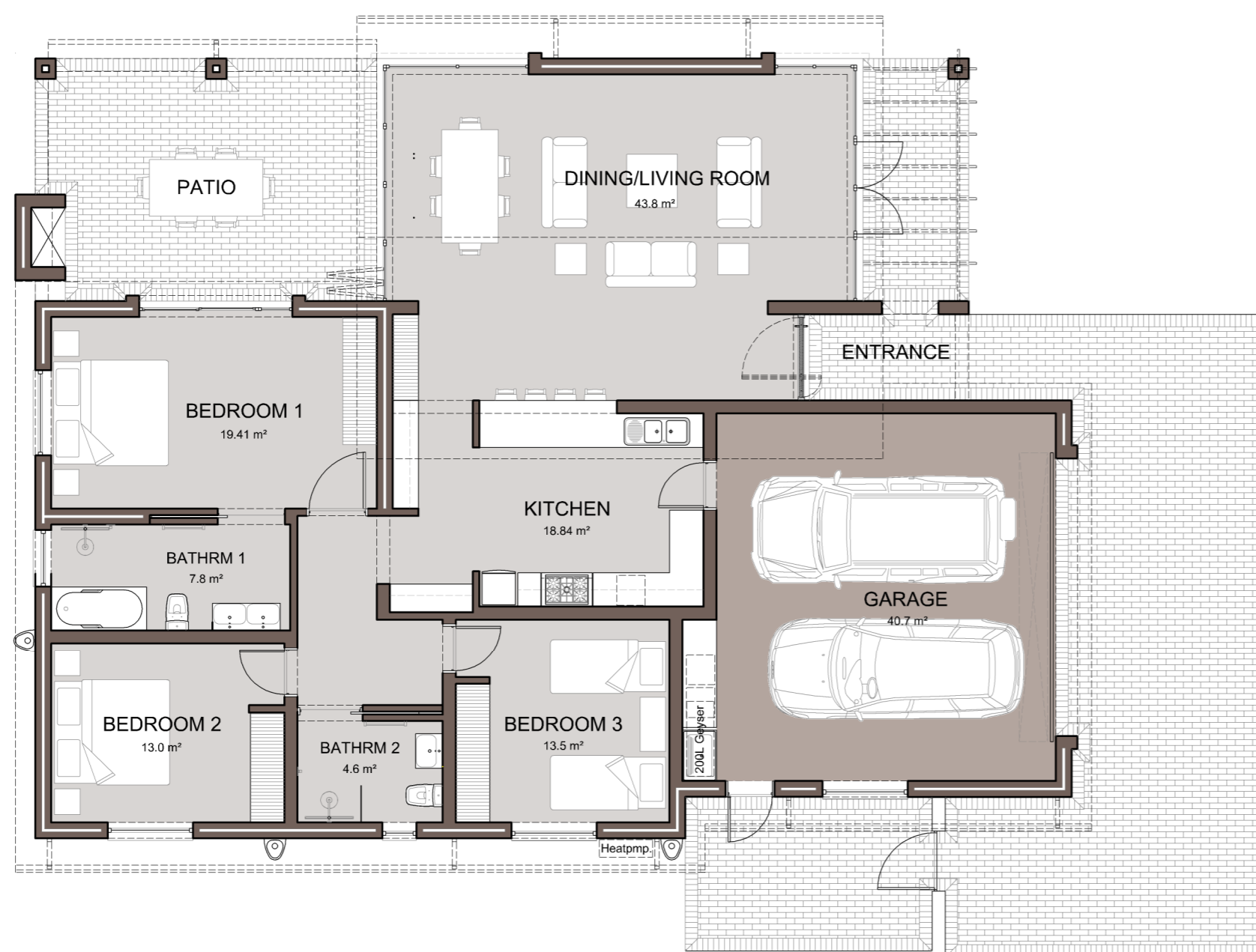
1: 100 FLOOR PLAN
