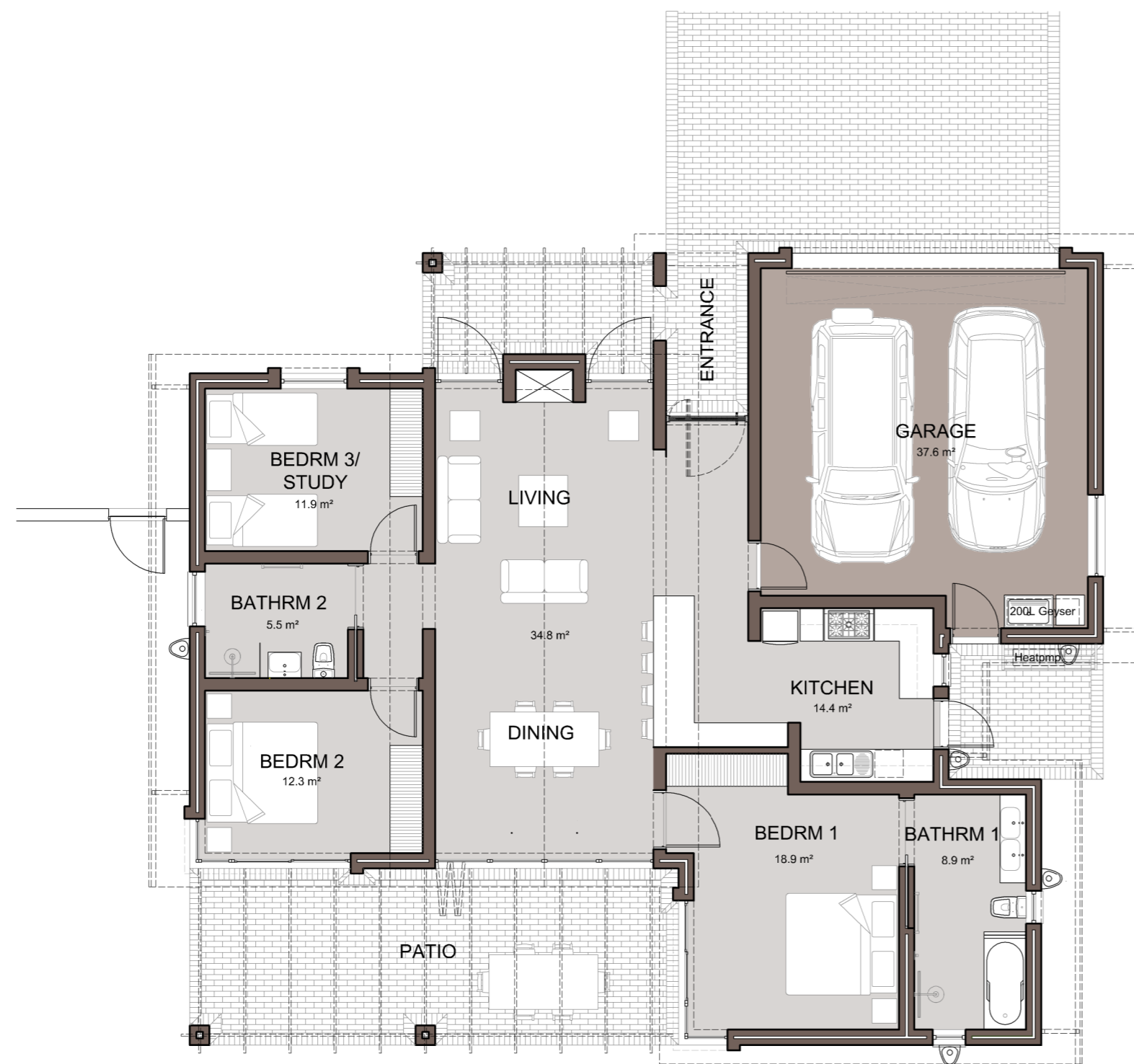
1: 100 FLOOR PLAN
