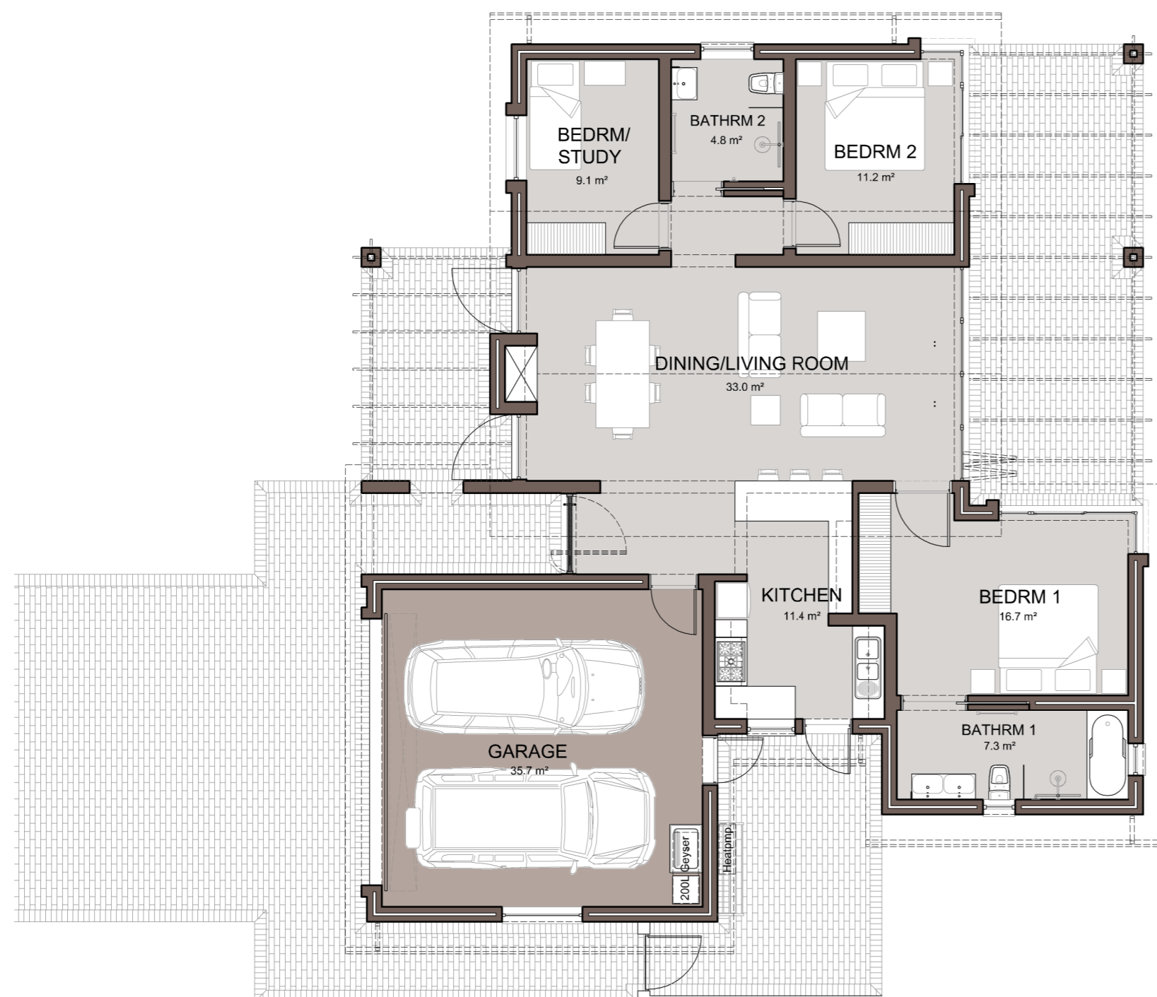
1: 100 FLOOR PLAN
