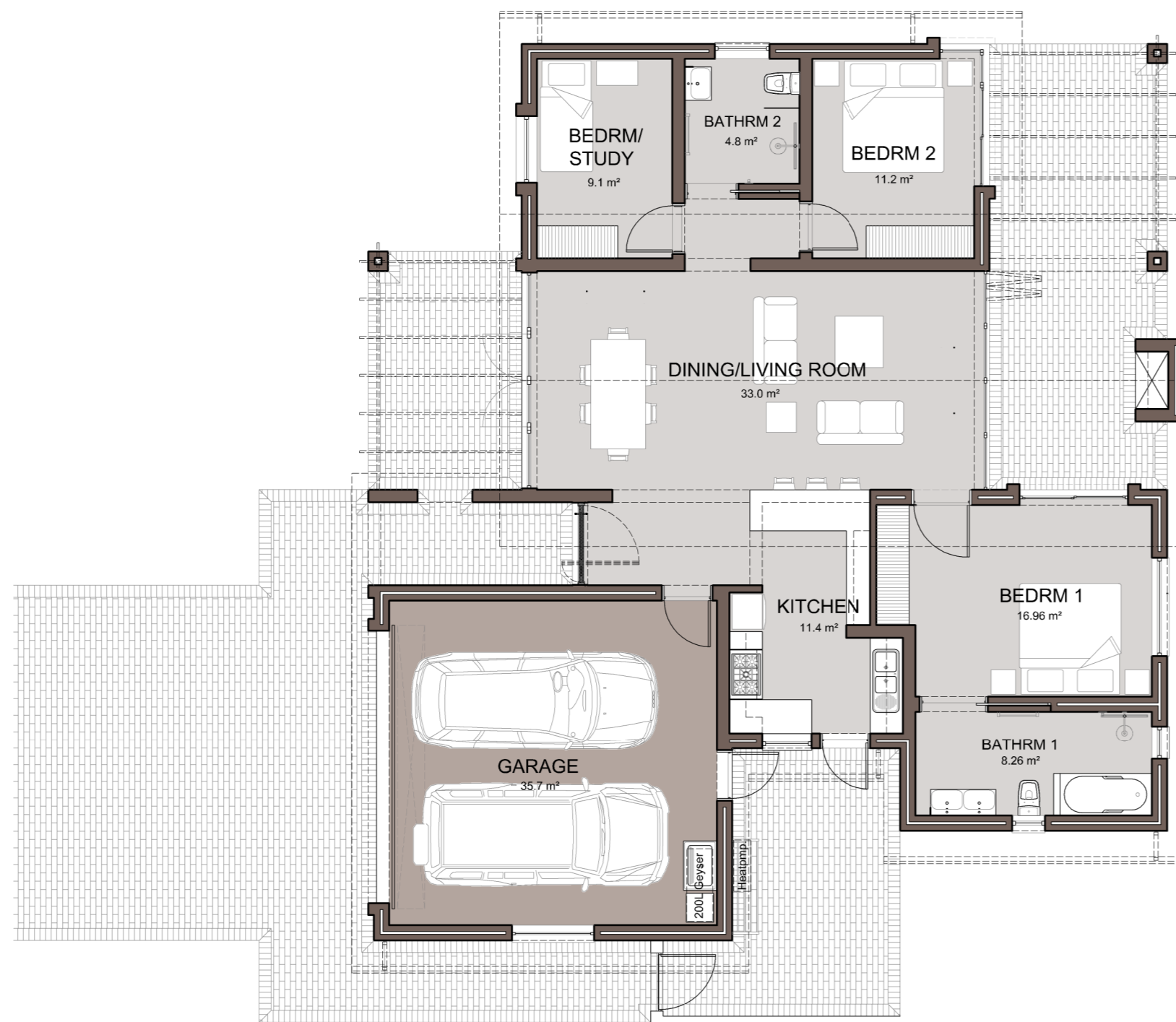
1: 100 FLOOR PLAN
